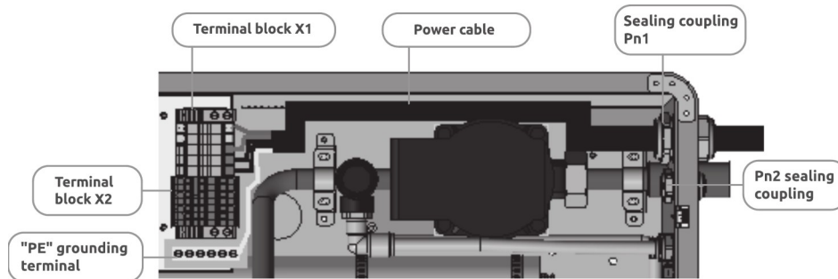
Figure 10 – Laying the power supply cable inside the boiler (the device is turned into a vertical view)
