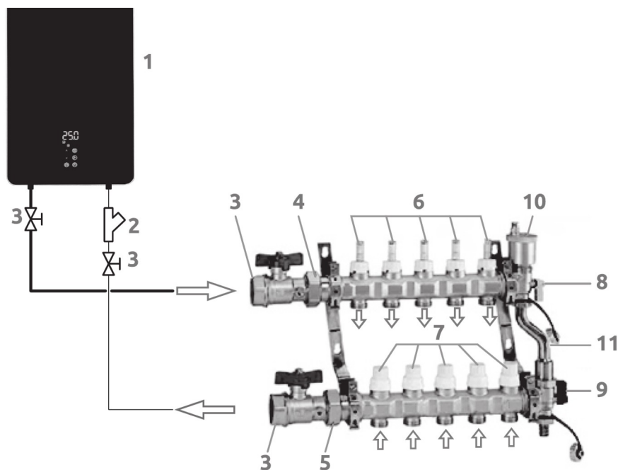
e 25 - Scheme of connecting the boiler to the underfloor heating sys
