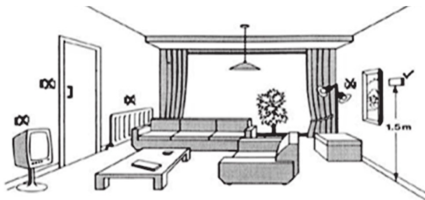
Installation in a room thermostat or air temperature sensor
